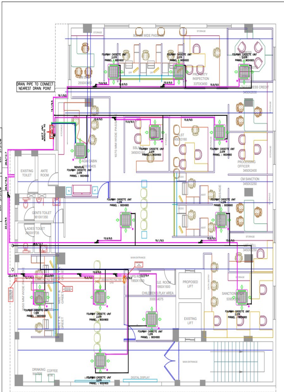
FIRST FLOOR HVAC PLAN
